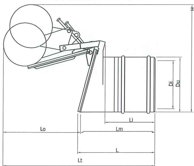
DN 100 – DN 200
